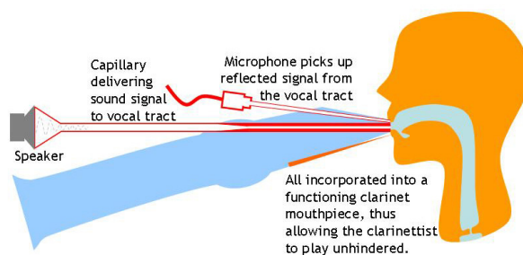
Figure 4. Schematic of the modified mouthpiece used in measuring the acoustic impedance of the player’s vocal tract.
