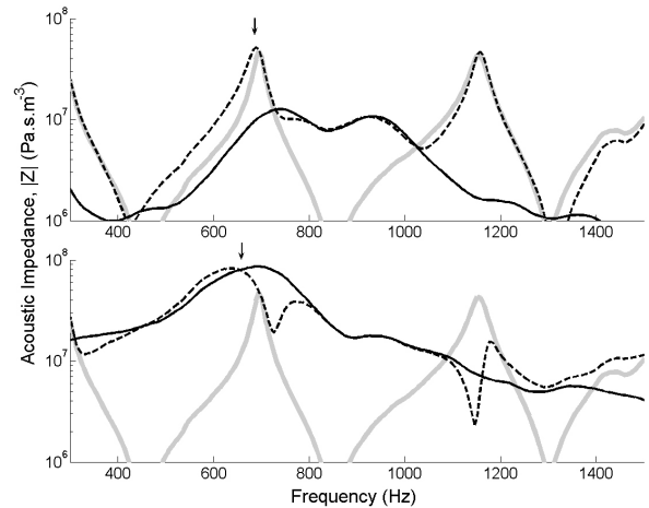
Figure 7. Measured impedance of clarinet (pale line), vocal tract (dark line) and combined impedance (dashed line). In both cases the fingered note is G5. Arrows indicate sounding pitch. In the top curve, the note is played normally. In the bottom curve, it is played as part of the glissando .
