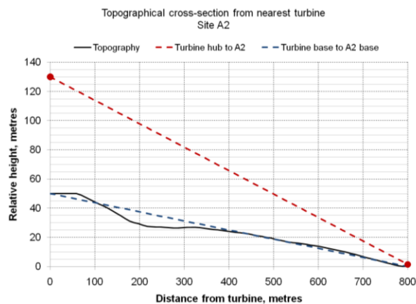
Figure 6. Topographical cross-section from nearest turbine to Site A2 (steady slope)
