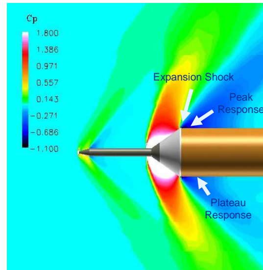
Figure 7. CFD visualization of C_p [7]
