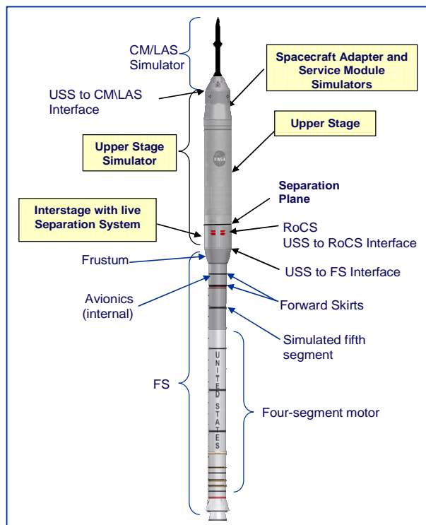
Figure 1. Ares I-X Flight Test Vehicle (FTV)
