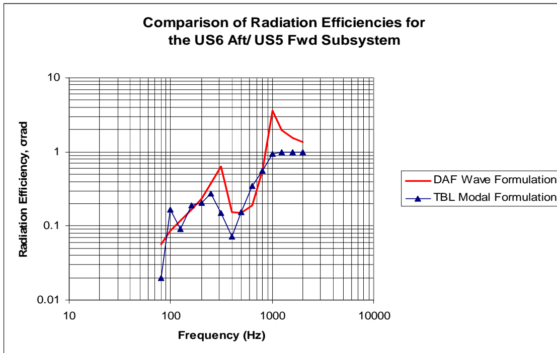
Figure 10. Radiation efficiencies for the US6 Aft/ US5 Fwd subsystem.
