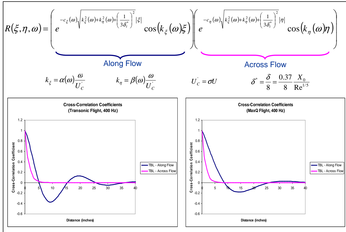
Figure 5. Turbulent boundary layer excitation definition [4]
