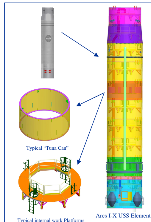
Figure 2. USS element description
