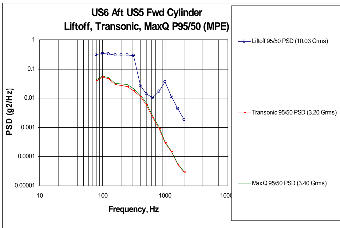
Figure 9. Typical tuna can structural response for lift-off, transonic and max Q excitations.
