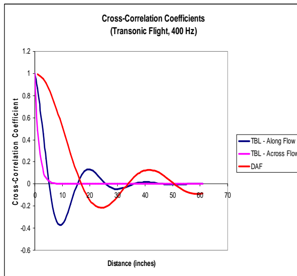
Figure 6. Comparison of DAF and TBL cross-correlation coefficients [4]
