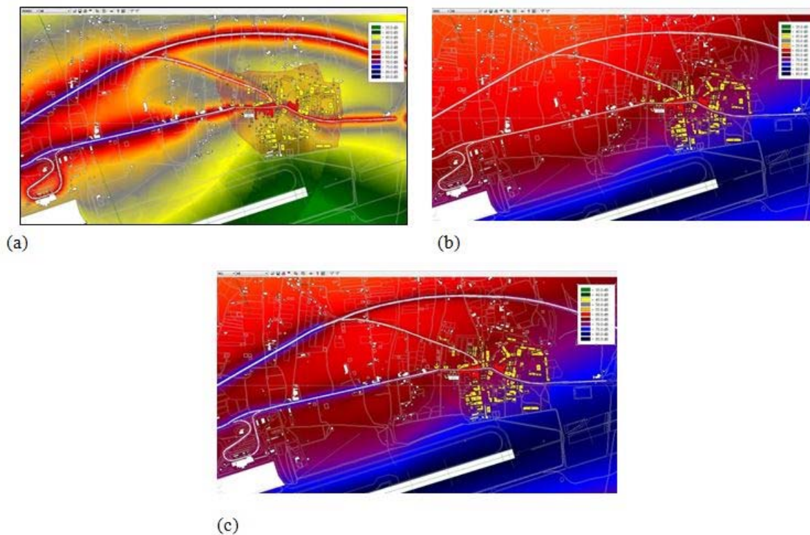
Figure 3 - Grid calculations for a combined noise situation (a) Traffic Noise Map, (b) Aircraft Noise Map and (c) Combined Noise Map (Aircraft + Road)
