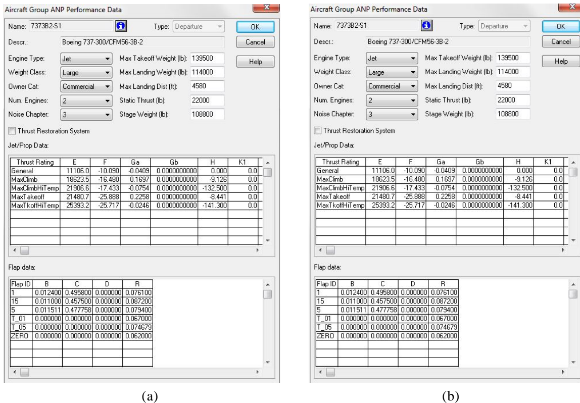
Figure 2 - (a) Aircraft group selected from the imported ANP database and (b) Performance data parameters
