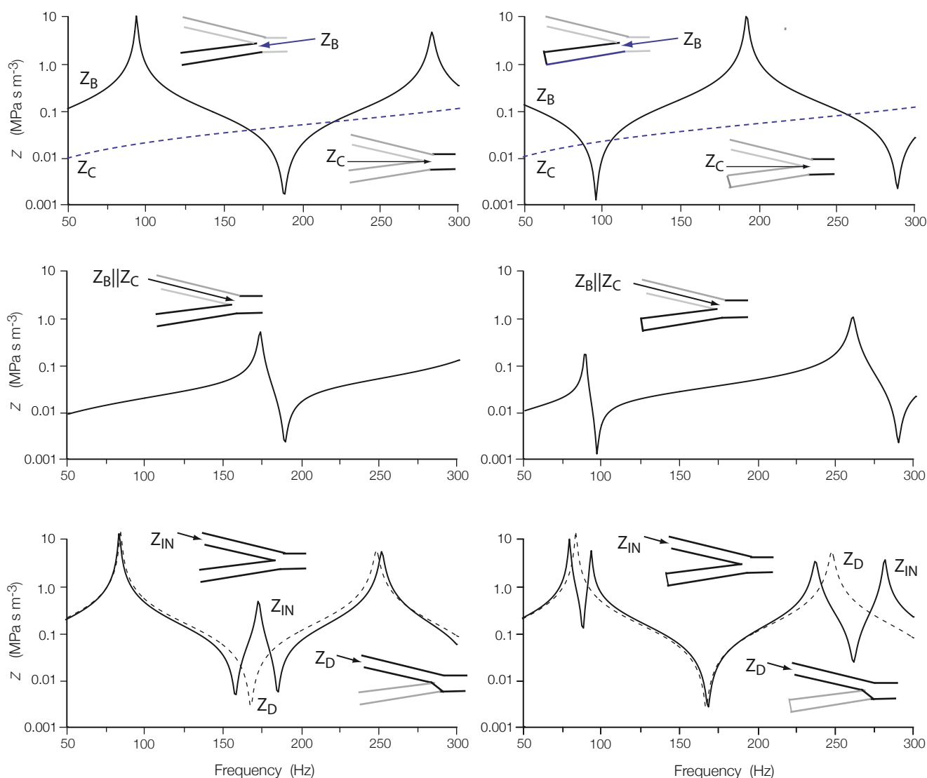
Figure 5. The calculated acoustic impedance of elements of the model shown in Fig. 2. The left and right hand curves were calculated with the end of tube B open or closed respectively. The continuous curves on the upper figures show the impedance Z_B of tube B alone as seen from the junction, whereas the dashed curves show the impedance Z_C of tube C alone as seen from the junction. The middle figures show the impedance Z_p presented at the junction by tube B and tube C in parallel. The lower curves show the input impedance Z_{IN} of the instrument when played at tube A. The dashed line on the lower curves shows the input impedance Z_D if tube B were blocked off at the junction.
