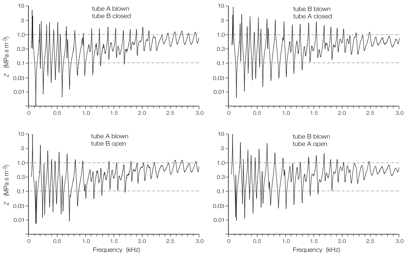
Figure 3. The measured acoustic input impedance Z_{IN} as a function of frequency plotted on a semi-logarithmic scale for the 4 possible input configurations of the forked didgeridu shown in Fig. 1.
