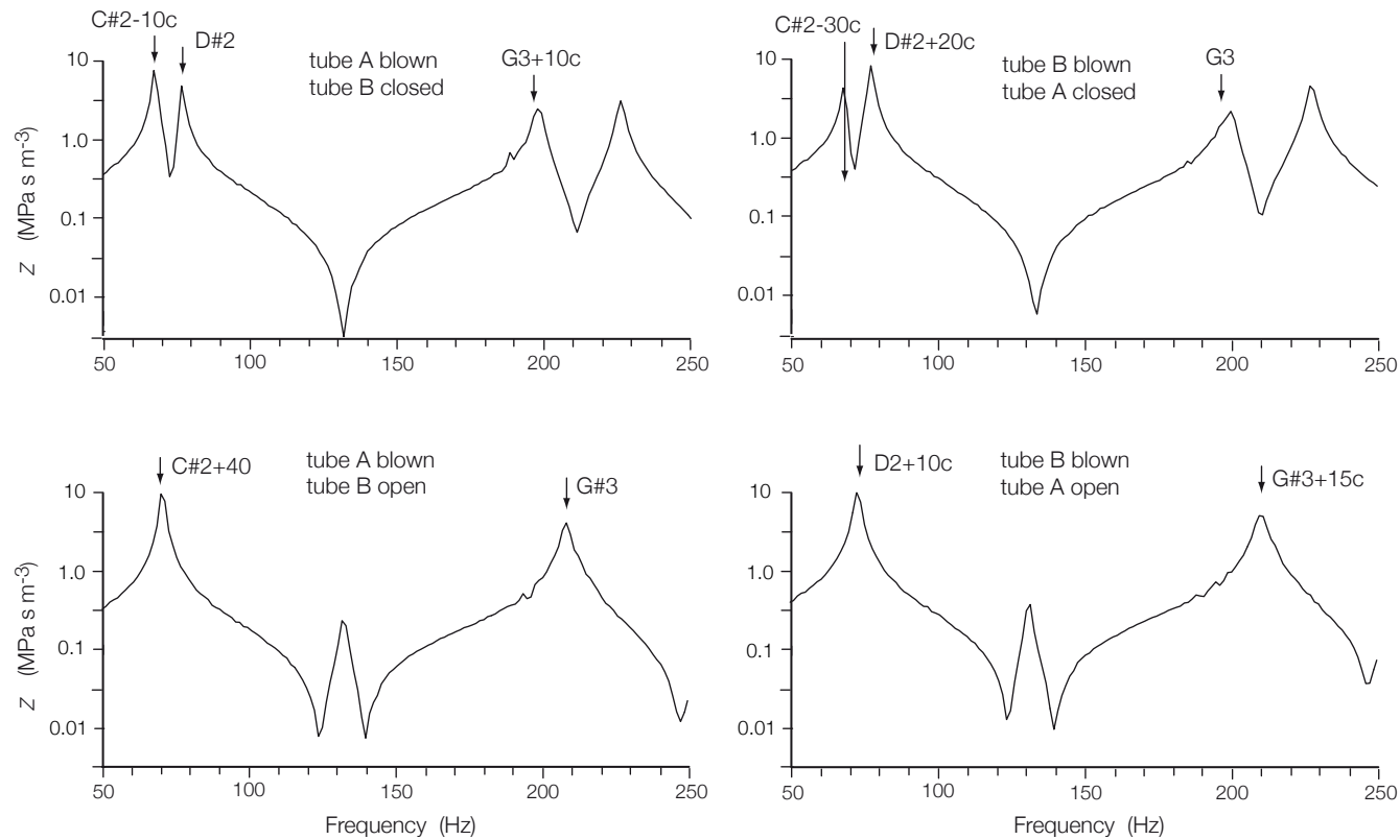
Figure 4. The measured acoustic impedance spectral data of Fig. 3 shown on an expanded scale for low frequencies. The vertical arrows indicate the frequencies of the musical notes played on the instrument by one of the investigators.
