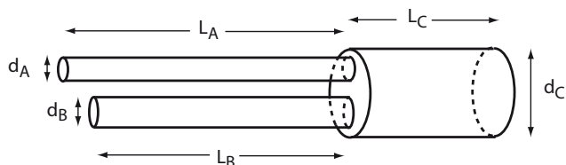
Figure 2. Schematic diagram used for the numerical model of the forked didjeridu measured in this study. Although the diameter d_C is greater than d_A + d_B in this sketch, this is not necessarily true in the model.
