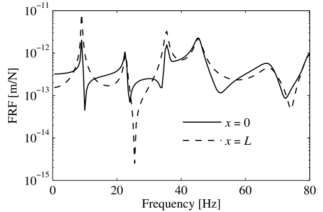
Figure 9. Frequency response of the radial displacement.
