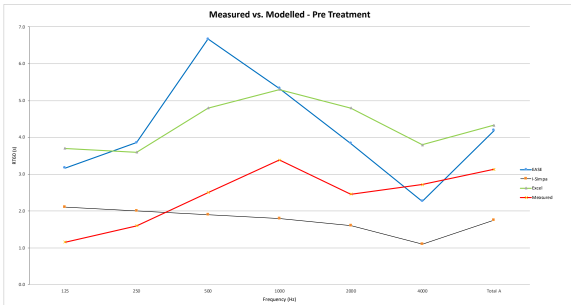
Modelled and Measured Comparison - Pre-treatment (RSA, 2018) Figure 5: Comparative Graph Pre-Treatment
