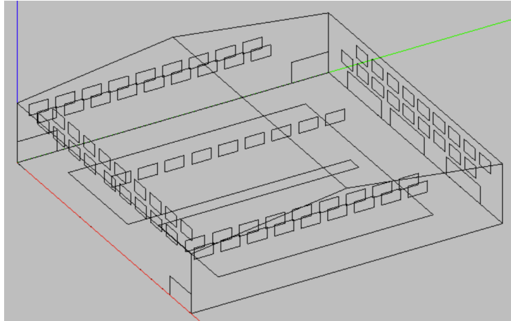
Floorplan (RSA, 2017) Figure 4: Hanging Baffle EASE modelling
