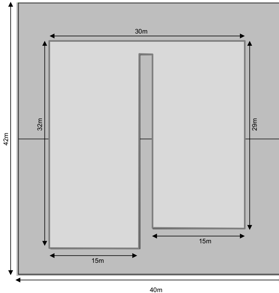
EASE Floorplan (RSA, 2017) Figure 1: EASE Floorplan
