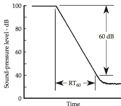
Master Handbook of Acoustics (F.Alton Everest & Ken C. Pohlmann, 2009) Figure 2: Measuring Reverberation Time
