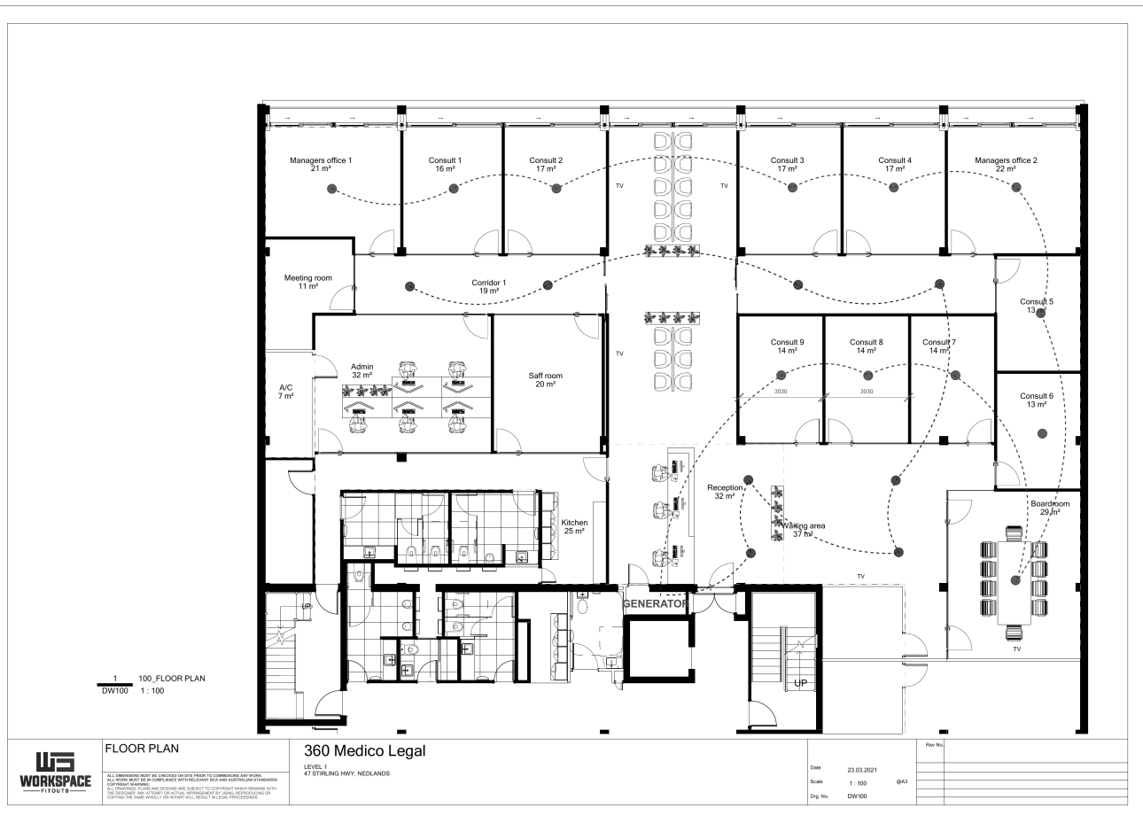
Figure 1: 360 Medico Legal sound mask system initial layout
