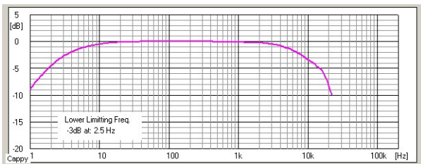
Figure 3. Diffuse-field response of a 1/2" free-field microphone
