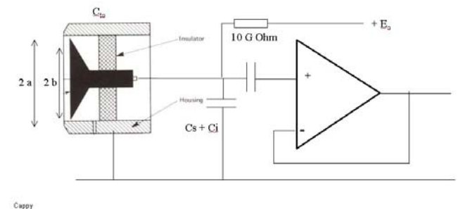
Figure 5. Principal schematic of a condenser microphone with pre-amplifier
