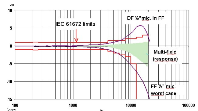
Figure 6. Multi-field FRF compared against IEC 61672 limits and 1/2" microphones (worst cases)
