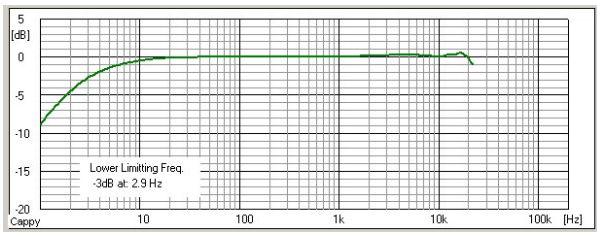
Figure 2. Free-field response of a 1/2" free-field microphone
