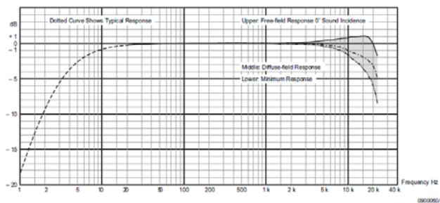
Figure 7. Multi-field Frequency responses: Free-field response (upper), Diffuse-field response (middle) and minimum response (lower)
