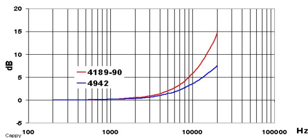
Figure 4. Maximal error for free-field microphone type 4189/90 (upper curve) and diffuse-field microphone type 4942 (lower curve)
