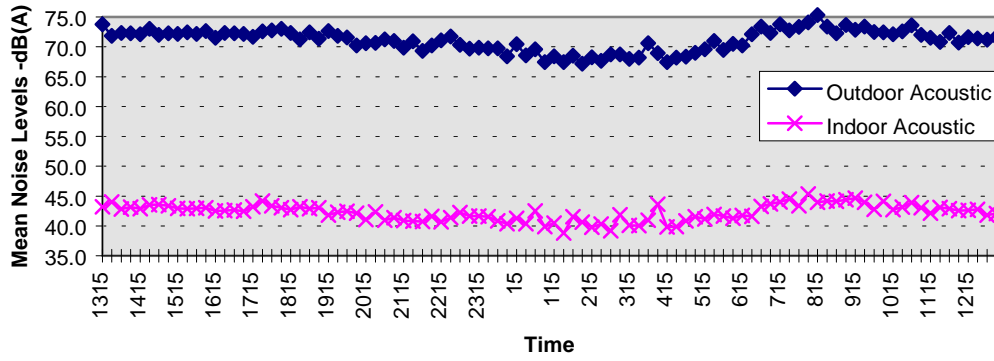
Figure 6 - Mean Outdoor and Indoor LA01 noise levels, acoustically designed dwelling, 15 minute intervals
