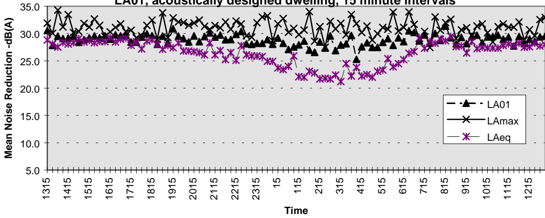
Figure 8 - 24 hour mean outdoor/indoor attenuation for LAeq, LAmx and LA01, acoustically designed dwelling, 15 minute intervals
