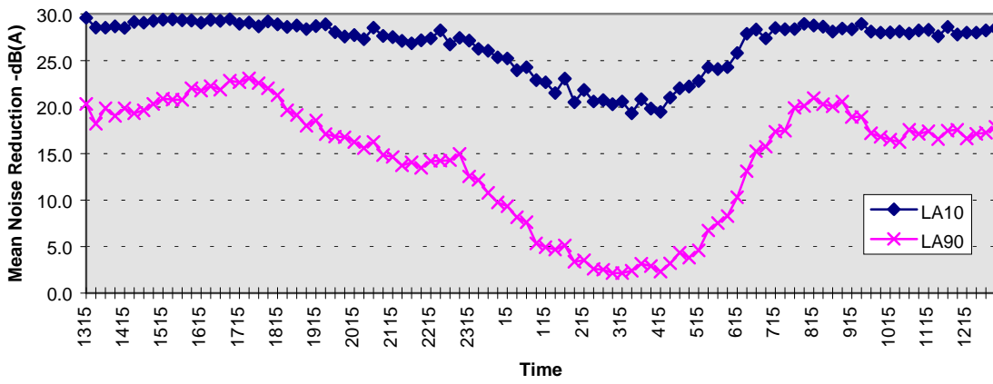
Figure 9 - 24 hour mean outdoor/indoor attenuation for LA10 and LA90, acoustically designed dwelling, 15 minute intervals
